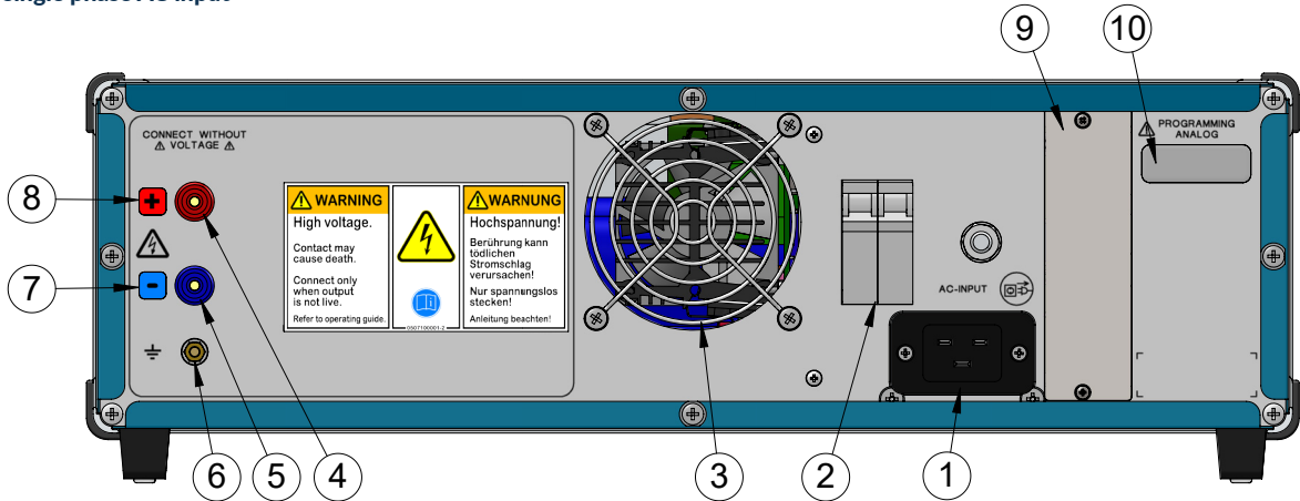
Rear view with single phase AC input
