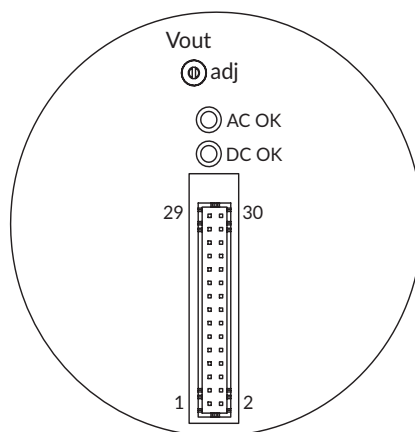
View A
