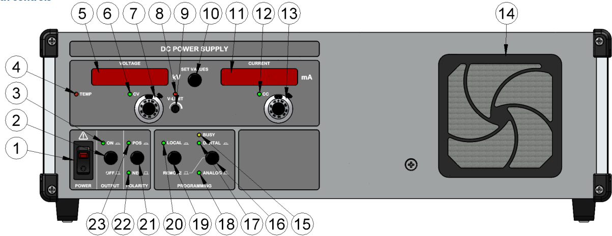
Front view with controls
