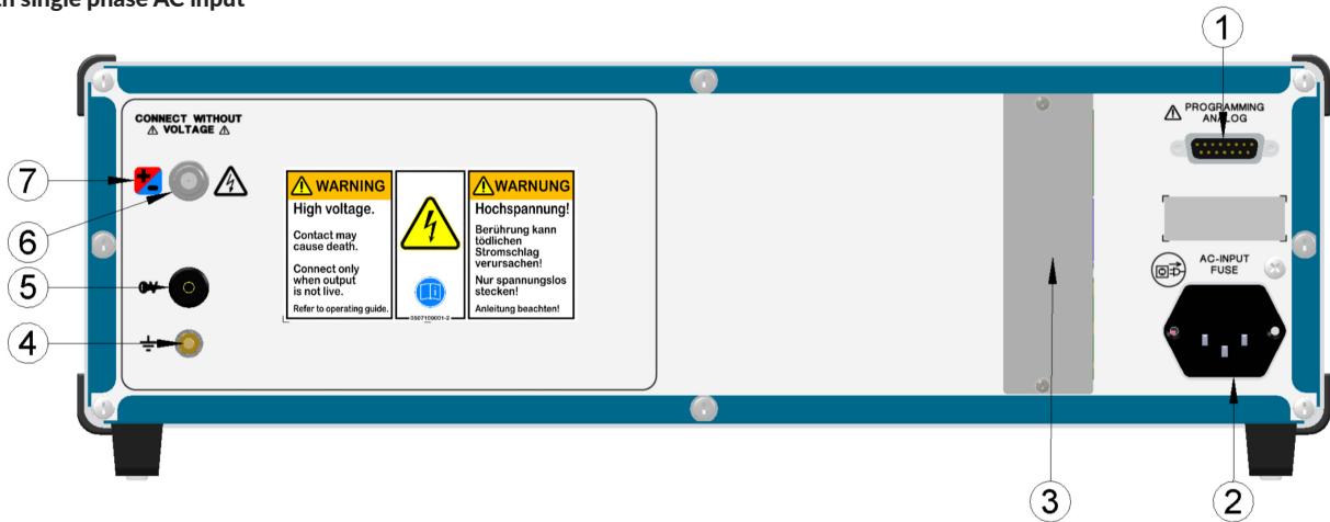
Rear view with single phase AC input
