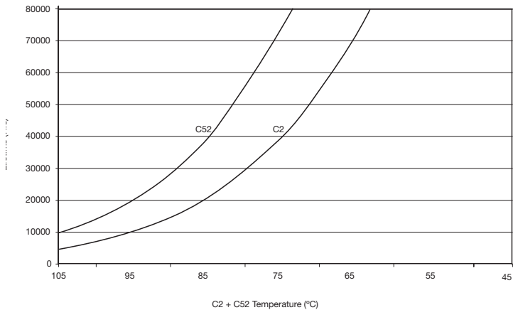
Estimate service life vs component temperature
