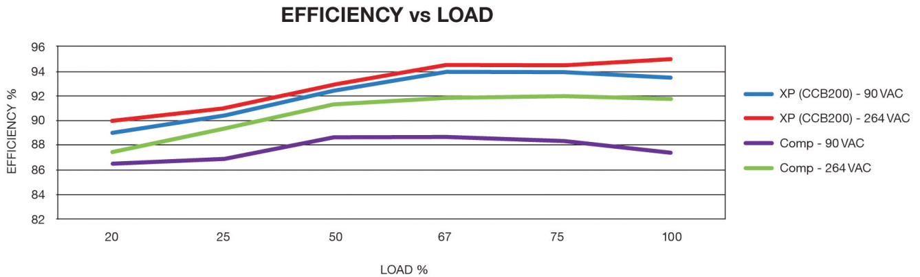
Figure 1 – Power supply efficiency over variable load conditions, with different supply voltages. Curves for the XP CCB200 and a comparable supply from another manufacturer are shown.
