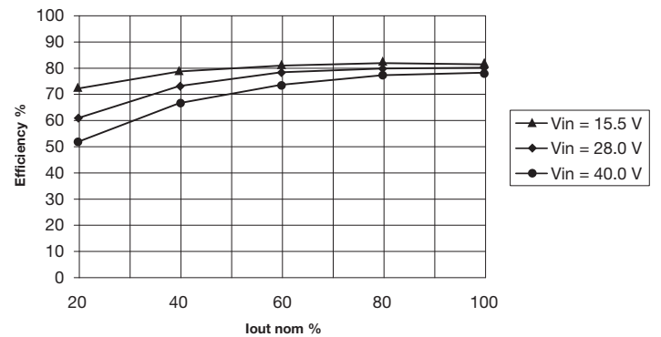
Figure 16. Typical efficiency for MTC0528S28
