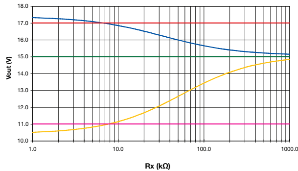
Figure 7. MTC0528S15 - Max and Min Adjustment
