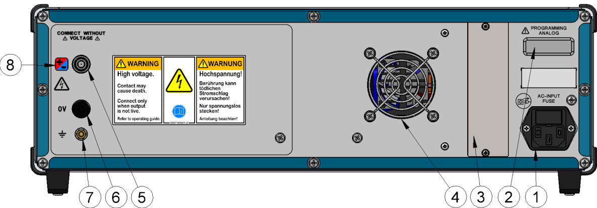
Example: HCP with polarity reversal and dimension: width 19"/443mm; height 3U/133mm
