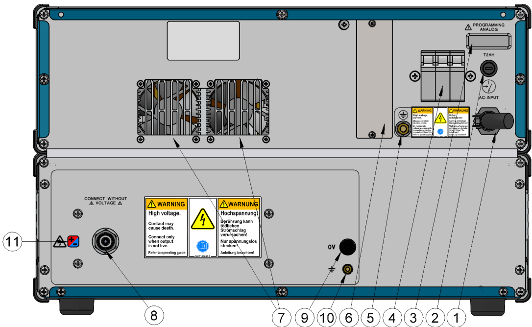
Example: HCP with polarity reversal and dimension: width 19"/443mm; height 6U/266mm
