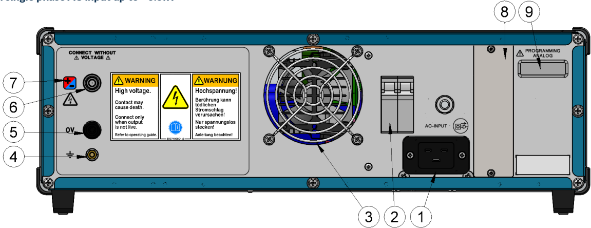
Rear view with single phase AC input up to +6.5kV
