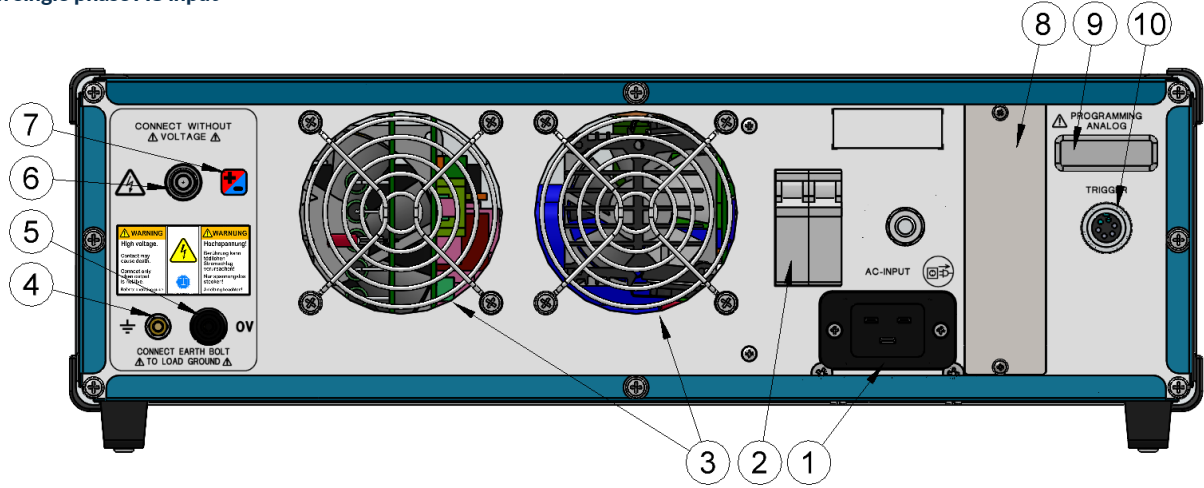
Example: HCK with polarity reversal and dimension: width 19"/443mm; height 3U/133mm
