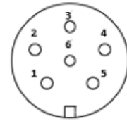
MINICON 6PIN (Solder side of the plug)
