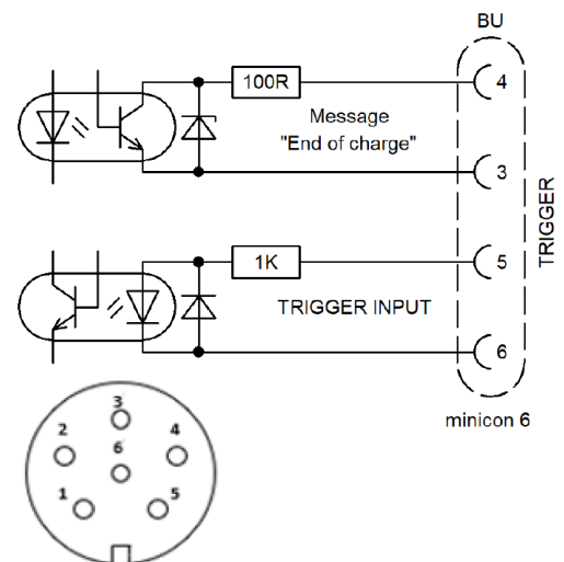
MINICON 6 pin (solder side of plug)
