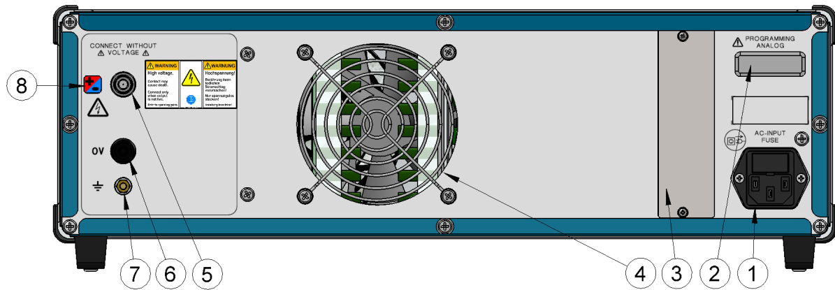
Example: HCB with polarity reversal and dimension: width 19"/443mm; height 3U/133mm
