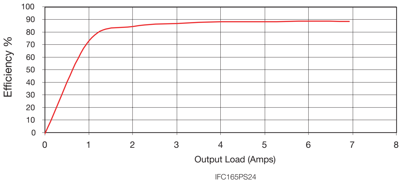
Efficiency against output load 230 VAC input
