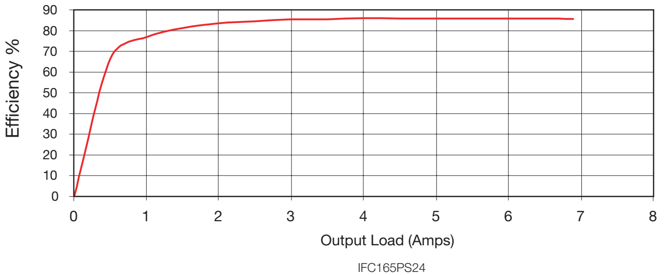
Efficiency against output load 115 VAC input
